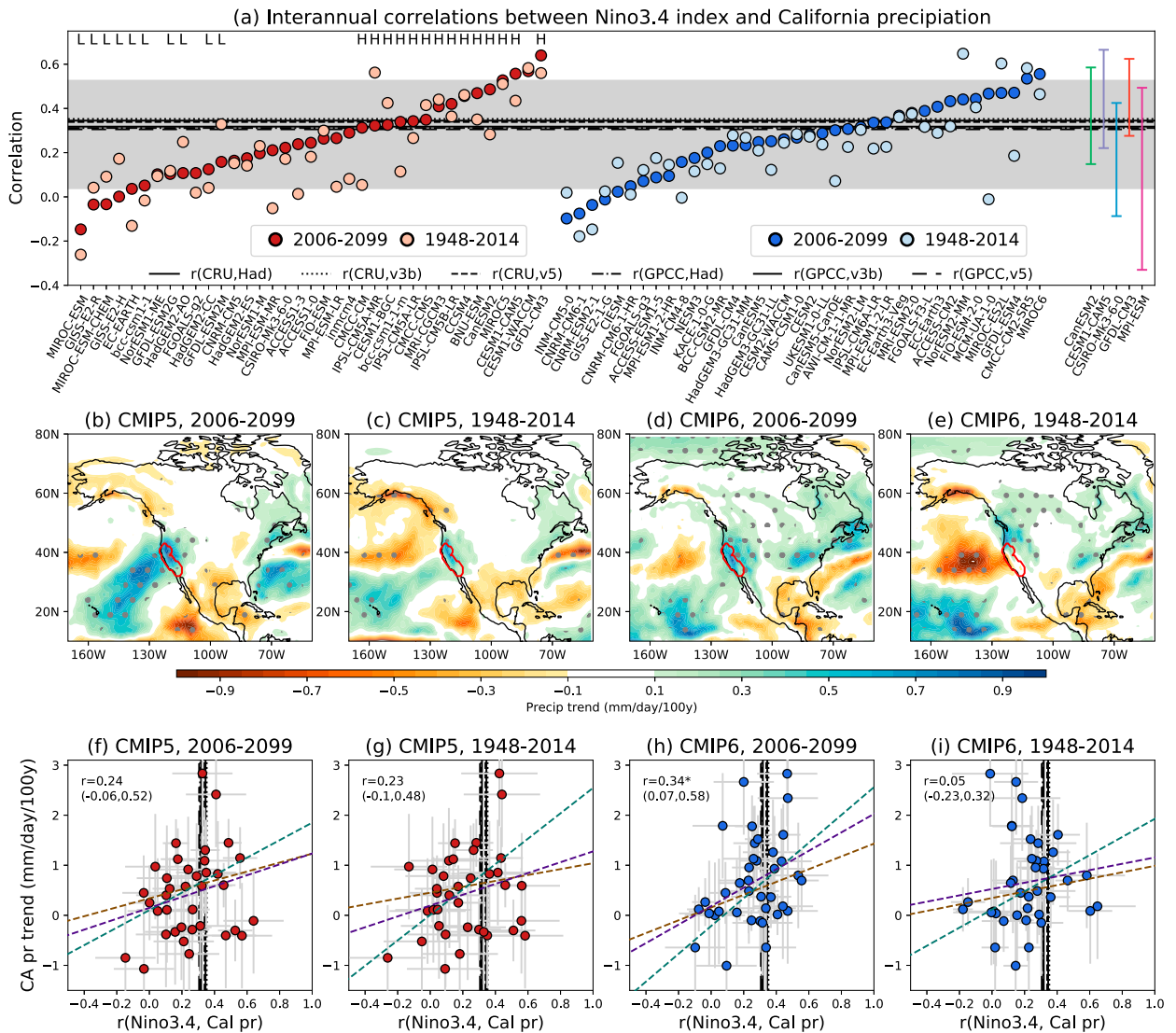
FIG. 13. (a) The interannual correlation between detrended DJF Niño-3.4 and detrended DJF California pr anomalies. Dark red and blue show CMIP5 and CMIP6 values using the 2006–99 period. Light red and light blue show the same but using the 1948–2014 period. Values are ordered according to the 2006–99 correlation, and the H’s and L’s depicted the models used in the “HIGH-r” and “LOW-r” composites of AL2017. Black lines show the correlation for different combinations of observational SST and precipitation datasets and the gray shading shows the 95% confidence interval on the correlation using GPCC precipitation and ERSSTv5 SSTs. Colored ranges on the right show the minimum to maximum range of the 1948–2014 correlations determined using the LEs. (b)–(e) Differences in 2006–99 precipitation trends between models with a correlation greater than 0.3 and those with a correlation less than 0.2. Stippling indicates regions where the difference is significant at the 95% level using a two-sided bootstrapping test. (f)–(i) The relationship between the 2006–99 precipitation trend over California and the correlation between the Niño-3.4 index and California precipitation. Correlations are quoted along with 95% confidence interval determined by bootstrapping models with replacement. Significant correlations are denoted by an asterisk. Titles in (b)–(i) indicate the time period used to calculate the correlation between the Niño-3.4 index and California precipitation.
