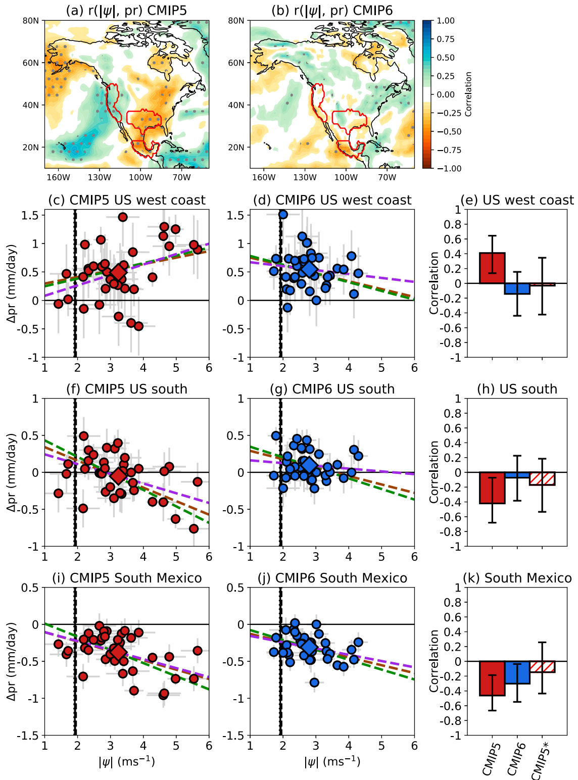
FIG. 11. (a),(b) The correlation between the stationary wave amplitude |\psi| and \Delta pr for CMIP5 and CMIP6 respectively. Stippled regions are significant at the 95% confidence level by a two-sided bootstrapping test and red contours depict the regions used in (c)–(k). (c),(d) The relationship between \Delta pr averaged over the U.S. west coast and |\psi| for CMIP5 and CMIP6 respectively along with |\psi| for the reanalyses and the best fitting linear regression (brown = OLS, green = TLS, purple = BHM). (e) The red and blue bars display the correlation and its 95% confidence interval (derived by bootstrapping models with replacement) of the points shown in (c) and (d), respectively, and the red hatched correlation, referred to as CMIP5*, shows the correlation across the CMIP5 models, excluding those that have |\psi| larger than the maximum |\psi| in CMIP6. (f)–(h) As in (c)–(e), but averaged over the U.S. South; (i)–(k) as in (c)–(e), but averaged over southern Mexico.
