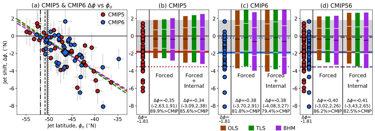
FIG. 5. (a) Jet shift ( \Delta\phi ) vs climatological jet latitude \phi_o for ensemble means of the CMIP5 (red) and CMIP6 (blue) models along with best fitting regression lines for CMIP5 and CMIP6 combined for OLS (brown), TLS (green), and BHM (purple). Black vertical lines show the reanalyses (see the legend of Fig. 2) and filled diamonds show the CMIP5 and CMIP6 ensemble means. (b) CMIP5 constrained projections: the left portion reproduces the CMIP5 \Delta\phi values of (a) along with the 66% confidence interval (dotted red lines); the middle portion shows the constrained projections for the forced response i.e., excluding internal variability; and the right portion shows the constrained projections for the forced response plus internal variability for a single realization. The red horizontal line across the panel shows the CMIP5 ensemble mean while the gray range shows the 95% confidence interval for the range of jet shifts that could arise due to internal variability for a single member, estimated from the LEs. (c) As in (b), but for CMIP6; (d) as in (b), but for CMIP5 and CMIP6 combined. Brown, green, and purple ranges with black line and white range show the 95% confidence intervals, mean, and 66% confidence intervals of constrained projections using TLS, OLS, and BHM, respectively. Values quoted are from the mean across the methods and are, from top to bottom, \Delta\phi , the range of the 95% confidence interval, and the probability of the real world future \Delta\phi being less poleward than the relevant CMIP ensemble mean.
