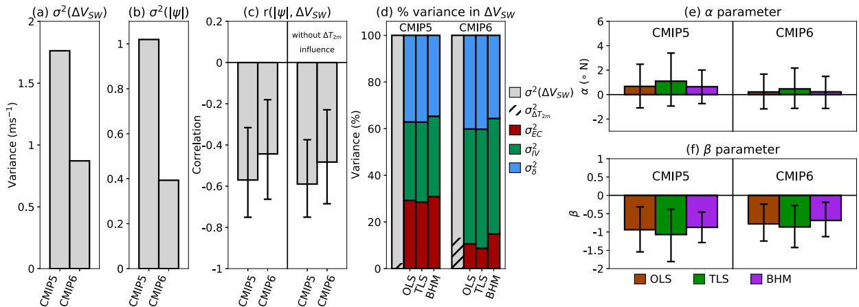
FIG. 8. (a) Variance in \Delta V_{sw} using the ensemble mean for each model. (b) As in (a), but for |\psi| . (c) The correlation between |\psi| and \Delta V_{sw} both without (left) and with (right) first regressing out the component that is linearly related to globally average surface temperature change \Delta T_{2m} . Whiskers show the 95% confidence interval derived by bootstrapping models with replacement. (d) A decomposition of the total variance in \Delta V_{sw} across models using a single member. The black hatching on the gray bar shows the percent variance explained by intermodel differences in \Delta T_{2m} , calculated by differencing the total variance and the variance after regressing out the contribution that is linearly related to \Delta T_{2m} . The colored bars show the percent variance explained by the EC (red), internal variability (green), and intermodel differences in the forced response that are unrelated to the EC (blue) for each method. (e),(f) The \alpha and \beta regression parameters for \Delta V_{sw} = \alpha + \beta|\psi| . Black ranges in (e) and (f) show the 95% confidence interval derived by bootstrapping models with replacement for OLS and TLS and by using the 1000 regression coefficients estimated from the BHM.
