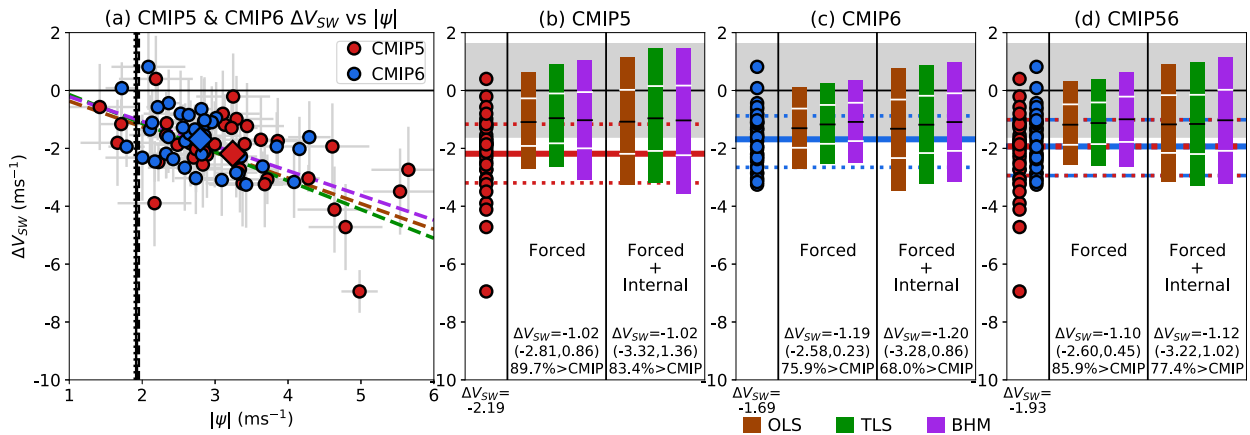
FIG. 10. (a) CMIP5 (red) and CMIP6 (blue) \Delta V_{sw} vs |\psi| along with the best fitting regression lines for CMIP5 and CMIP6 combined using OLS (brown), TLS (green), and BHM (purple). The four reanalyses are shown by the black lines (see Fig. 7 legend). (b) The left portion of the panel reproduces the CMIP5 \Delta V_{sw} from (a) and the red line that spans the panel shows the CMIP5 ensemble mean. The gray shaded region shows the 95% confidence interval of anomalies in \Delta V_{sw} that could arise due to internal variability, determined from the LEs. In the middle portion of the panel, the colored bars show the 95% confidence interval of the constrained forced response using OLS (brown), TLS (green), and BHM (purple). The black line shows the mean of the constrained distribution and white lines delineate the 66% confidence interval on the constrained distribution. The right portion of the panel is the same as the middle but including the contribution to \Delta V_{sw} from internal variability that could arise in our one future. Numbers quoted are, from top to bottom, the mean across the methods of the mean change in \Delta V_{sw} , the 95% confidence interval of the constrained distribution (c), and the probability that \Delta V_{sw} will be greater than (less negative) than the CMIP ensemble mean. (c), (d) As in (b), but for CMIP6 and for CMIP5 and CMIP6 combined, respectively.
