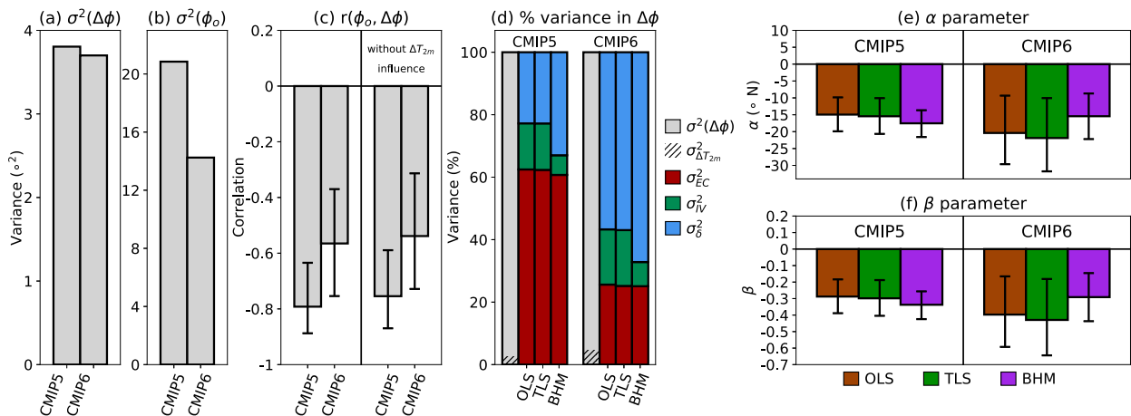
FIG. 3. (a) Variance in \Delta\phi using ensemble means for each model. (b) As in (a), but for \phi_o . (c) The correlation r between \phi_o and \Delta\phi both without (left) and with (right) first regressing out the component that is linearly related to globally averaged surface temperature change ( \Delta T_{2m} ). Whiskers show the 95% confidence intervals estimated using a bootstrapping with replacement procedure. (d) A decomposition of the total variance across models, using a single member. The black hatching on the gray bar shows the percent variance explained by intermodel differences in \Delta T_{2m} , calculated by differencing the total variance and the variance after regressing out the contribution that is linearly related to \Delta T_{2m} . The colored bars show the percent variance explained by the EC (red), internal variability (green), and intermodel differences in the forced response that are unrelated to the EC (blue) for each method. (e),(f) The \alpha and \beta regression parameters. Black ranges in (e) and (f) show the 95% confidence intervals derived by bootstrapping models with replacement for OLS and TLS and by using the 1000 estimates of the regression coefficients from the BHM.
