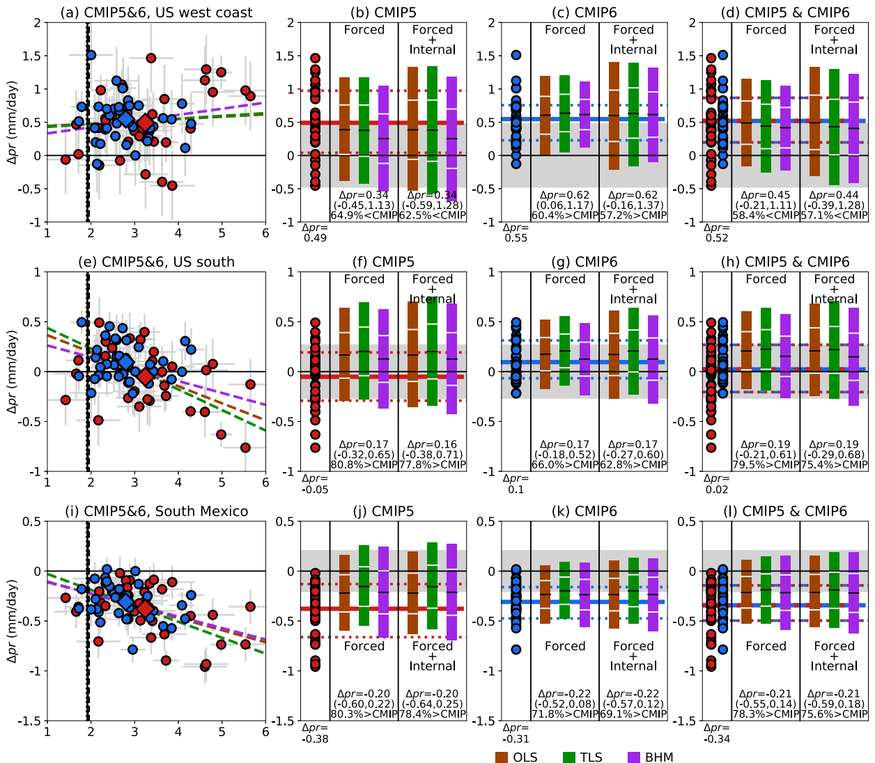
FIG. 12. (a) The relationship between \Delta pr averaged over the U.S. west coast and |\psi| (red circles = CMIP5, blue circles = CMIP6, red diamond = CMIP5 mean, blue diamond = CMIP6 mean, black vertical lines = the reanalyses |\psi| , brown green, and purple dashed lines = the OLS, TLS, and BHM regression lines using CMIP5 and CMIP6 combined). (b) The CMIP5 \Delta pr averaged over the U.S. west coast (shown at left), the constrained distributions of the forced change (shown at center), and the constrained distribution of the forced change + internal variability (shown at right). Colored bars show the 95% confidence interval of the constrained distribution; the black line shows the mean, and white range shows the 66% confidence interval. Red lines spanning the panel show the CMIP5 ensemble mean and 66% confidence interval, and the gray range shows the 95% confidence range of \Delta pr values that could arise due to internal variability. (c) As in (b), but for CMIP6; (d) as in (b), but for CMIP5 and CMIP6 combined. (e)–(h) As in (a)–(d), but averaged over the U.S. south. (i)–(l) As in (a)–(d), but averaged over southern Mexico. The values quoted are, from top to bottom, the mean across the methods of the mean \Delta pr , the 95% confidence interval of the constrained distribution (ci), and the probability, from the constrained distribution, that the \Delta pr will be greater than or less than the CMIP5 or CMIP6 ensemble mean (whichever is larger).
