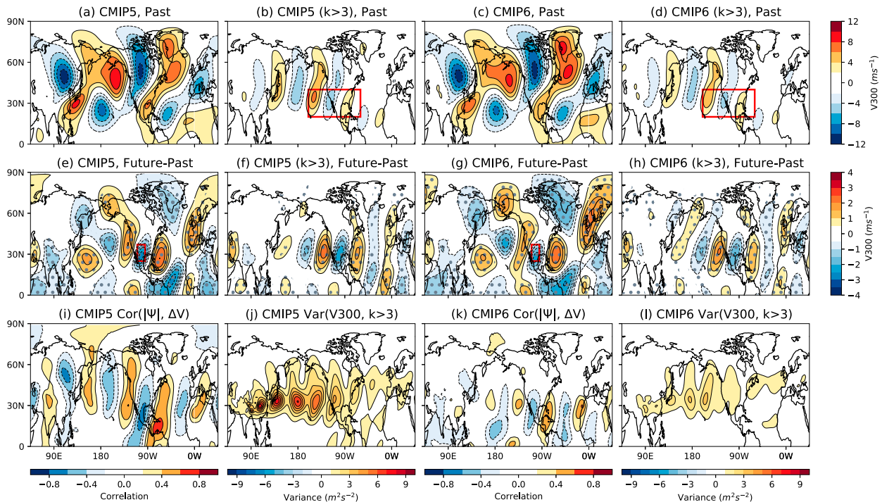
FIG. 6. A comparison of 300-hPa meridional wind between (left) CMIP5 and (right) CMIP6. (a),(c) The climatological V300 for CMIP5 and CMIP6, respectively; (b),(d) as in (a) and (c), but after filtering to only retain zonal wavenumbers greater than 3. (e),(g) The future – past difference for CMIP5 and CMIP6, respectively; (f),(h) as in (e) and (g), but after filtering to only retain zonal wavenumbers greater than 3. (i),(k) The correlation between the climatological k > 3 stationary wave amplitude ( |\psi| ) and the change in 300-hPa meridional wind across models for CMIP5 and CMIP6. (j),(l) The across-model variance in k > 3 meridional wind for CMIP5 and CMIP6, respectively. The stippling in (e)–(h) shows regions where more than 80% of the models agree on the sign of the anomaly. The red box in (b) and (d) shows the region used to define |\psi| ( 160^{\circ} – 60^{\circ} W, 20^{\circ} – 40^{\circ} N). The red box in (e) and (g) shows the region used to define \Delta V_{sw} ( 110^{\circ} – 95^{\circ} W, 25^{\circ} – 37^{\circ} N).
